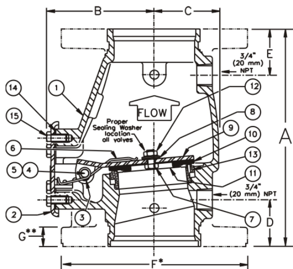
Figure 1 Model J-1 Alarm Check Valve
