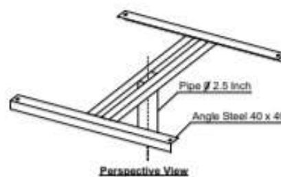
DET. Solar Panel Bracket Scale 1 : -
