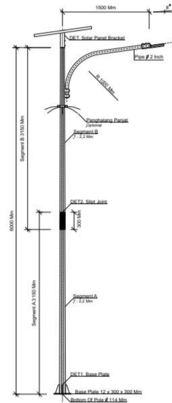
TIANG PJUTS 2 IN 1 OCTAGONAL 6 METER Scale 1 : 40 - Octagonal -
