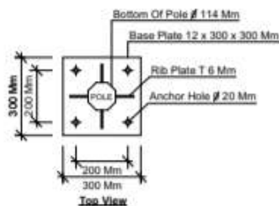
DET1. Base Plate Scale 1 : -
