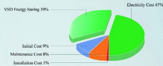
VSD Compressor
