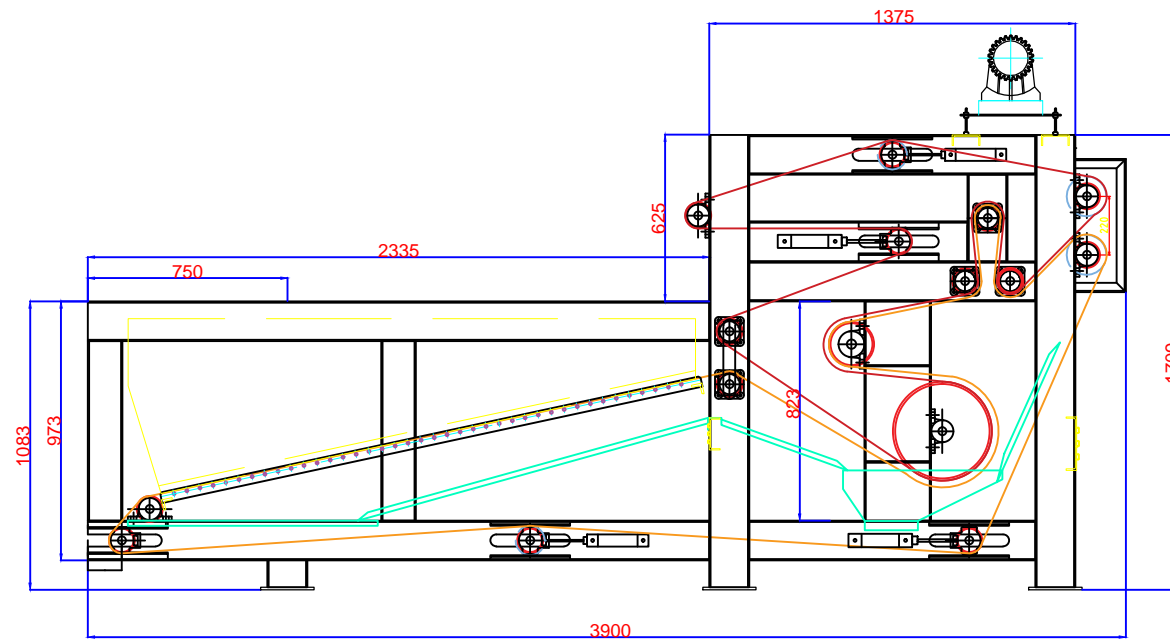
TAMPAK SAMPING
