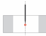
Measurement of internal diameter by using single arm measuring attachment with one axis bi-directional probing
