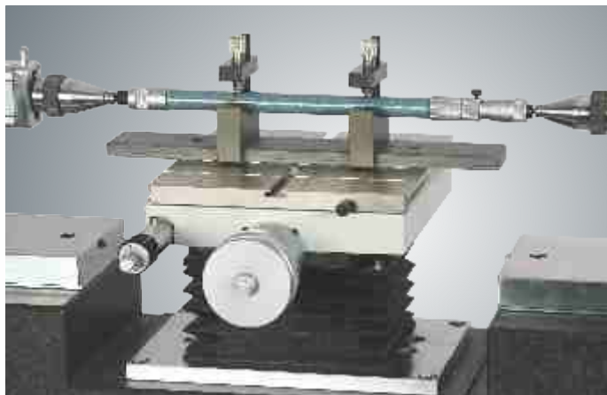
Internal Micrometer (2 point) Calibration : Hold on table by using holding attachment
