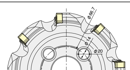
Fig.3 (エア穴無し) (Without air hole)
