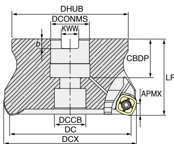
Fig.1 (エア穴付き) (With air hole)
