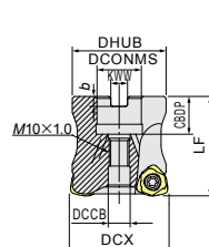
Fig.1 (エア穴付き) With air hole
