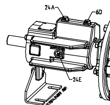
Version with double-acting mechanical seal
