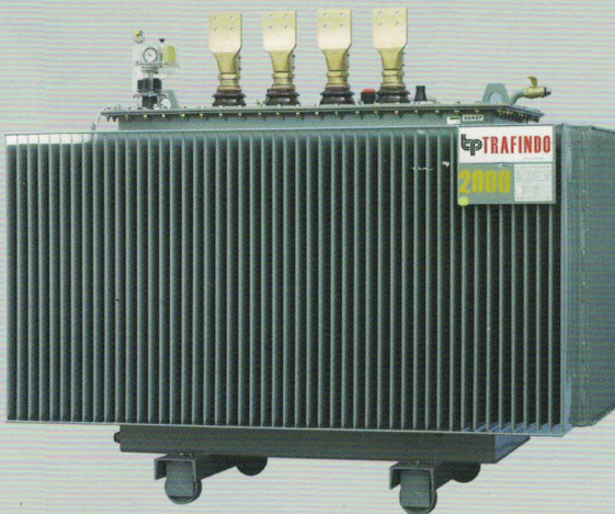
Hermetically-sealed type
