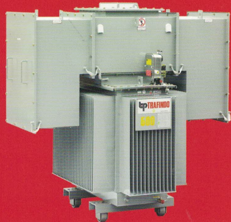
Hermetically-sealed type with cable termination boxes
