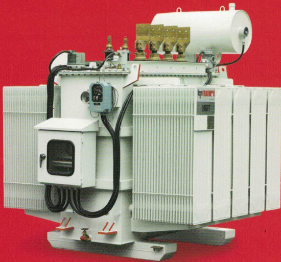
Conservator type
