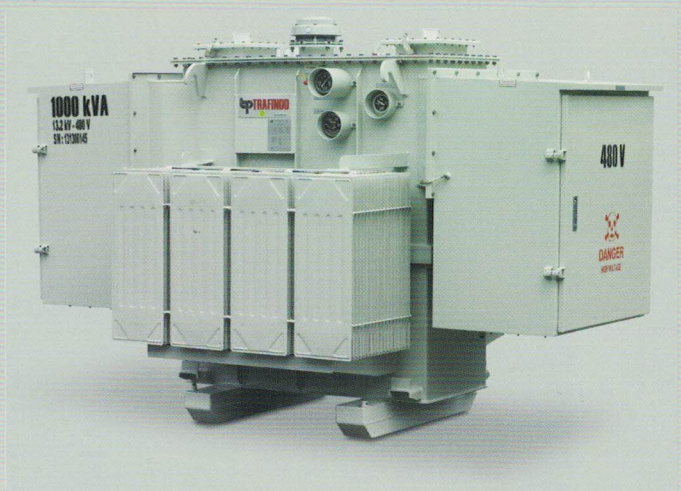
Hermetically-sealed type with nitrogen cushion
