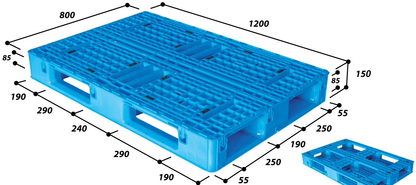
Bottom View
