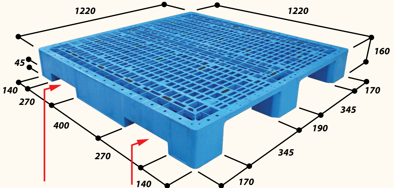
Notched design for safe beam racking & fork entry
