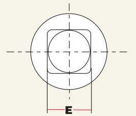
MODEL STM10-STM52 OUTPUT SHAFT
