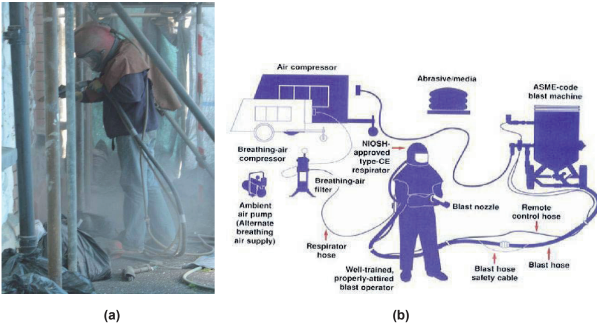
Figure 2 (a) Grit blast working environment/application, and (b) typical equipment/apparatus required for carrying out grit blast process.
