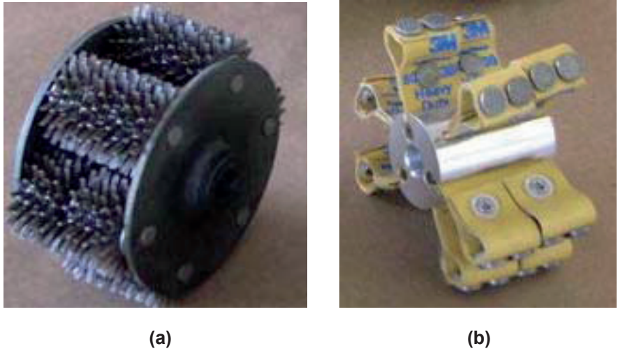
Figure 7 (a) Typical cutter bundle surface preparation tool comprised of 6 rows of spur-like hardened steel discs, and (b) rotary flap surface preparation tool consisting of 6 equally spaced rows of multi-faceted tungsten carbide shot.
