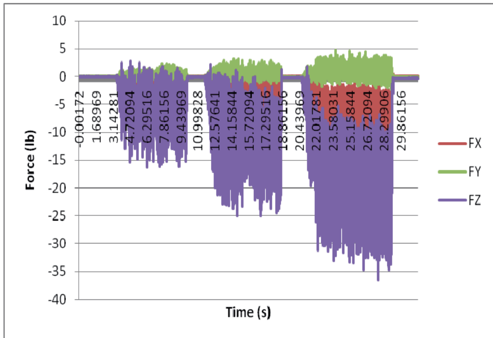
Figure 5 Measured vibratory force generated by needle gun when exerted against vertical steel surface during typical surface cleaning exercise. Three different levels of force exertion, namely, low (left), medium (center), and high (right) were used during the cleaning operation [6]. (API 5L steel, air supply pressure 100 psi, angle of inclination \alpha \approx 60 degrees). Results exclude the weight of the needle gun (15 N [3.5 lb]).
