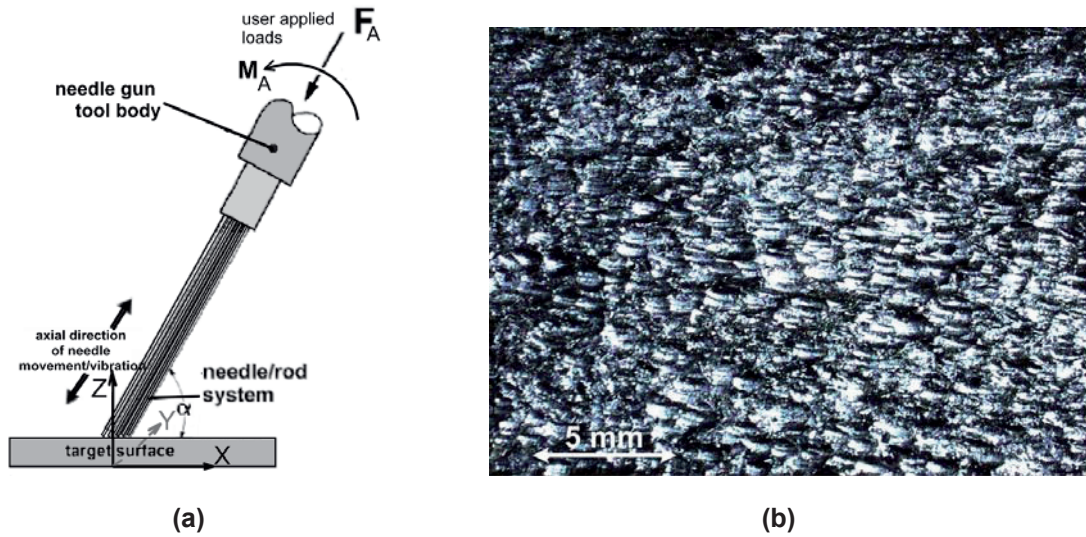
Figure 3 (a) Schematic of needle gun depicting user-applied force F_A and moment M_A , tool orientation angle \alpha , and axial mode of vibratory oscillating rods, and (b) typical surface texture generated by repetitive contact of rod tips with target surface. Elliptic micro-indentations are indicative of corner contact made between wire rods and target surface.
