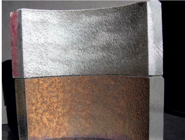
Figure 16 Interior of API 5L piping in as-received condition (bottom), and after bristle blast cleaning (top).
