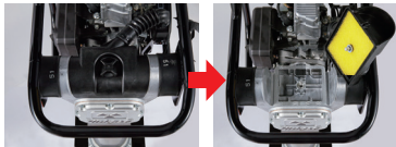
● Pre-cleaner combined with crank case
