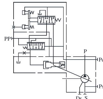
Constant Power Control Type With External Pilot
