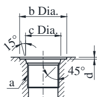
Detail of Port
