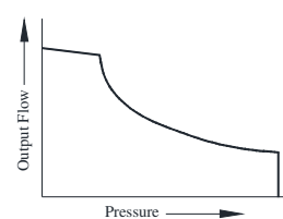
Constant Power Control Type Constant Power Control Type With External Pilot
