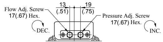
View Arrow X
