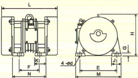
Dimension sketch
