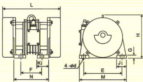
Dimension sketch
