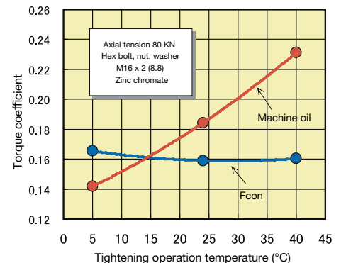
Influence of temperature on torque coefficient
