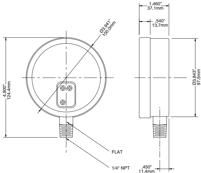
4" Bottom Connection
