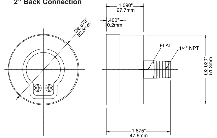
2" Back Connection
