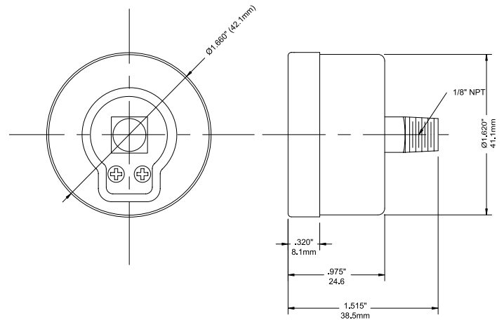
1.5" Back Connection
