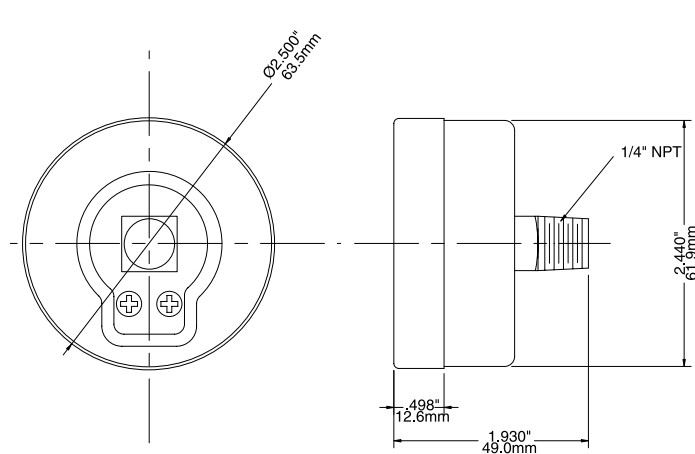
2.5" Back Connection
