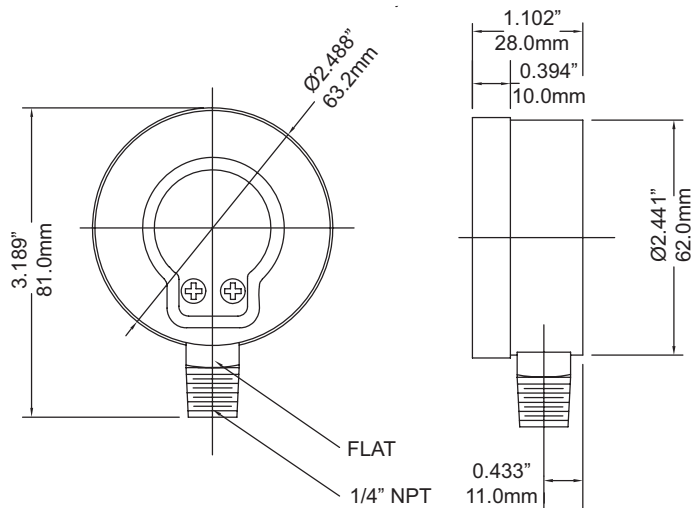
2.5" Bottom Connection
