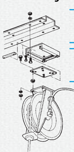
N372407 RK-W Wall mounting swing bracket (SPCC)
