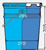
Open Head Tapered Pail
