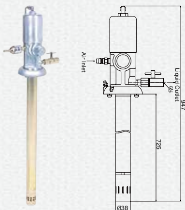
880846 SKR-725A55 Drum Pump for 55kg(120lb) Drum
