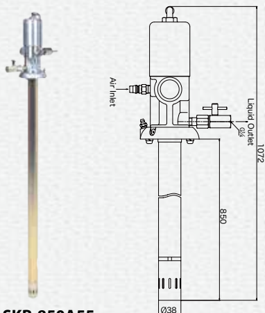
880847 SKR-850A55 Drum Pump for 180kg(400lb) Drum
