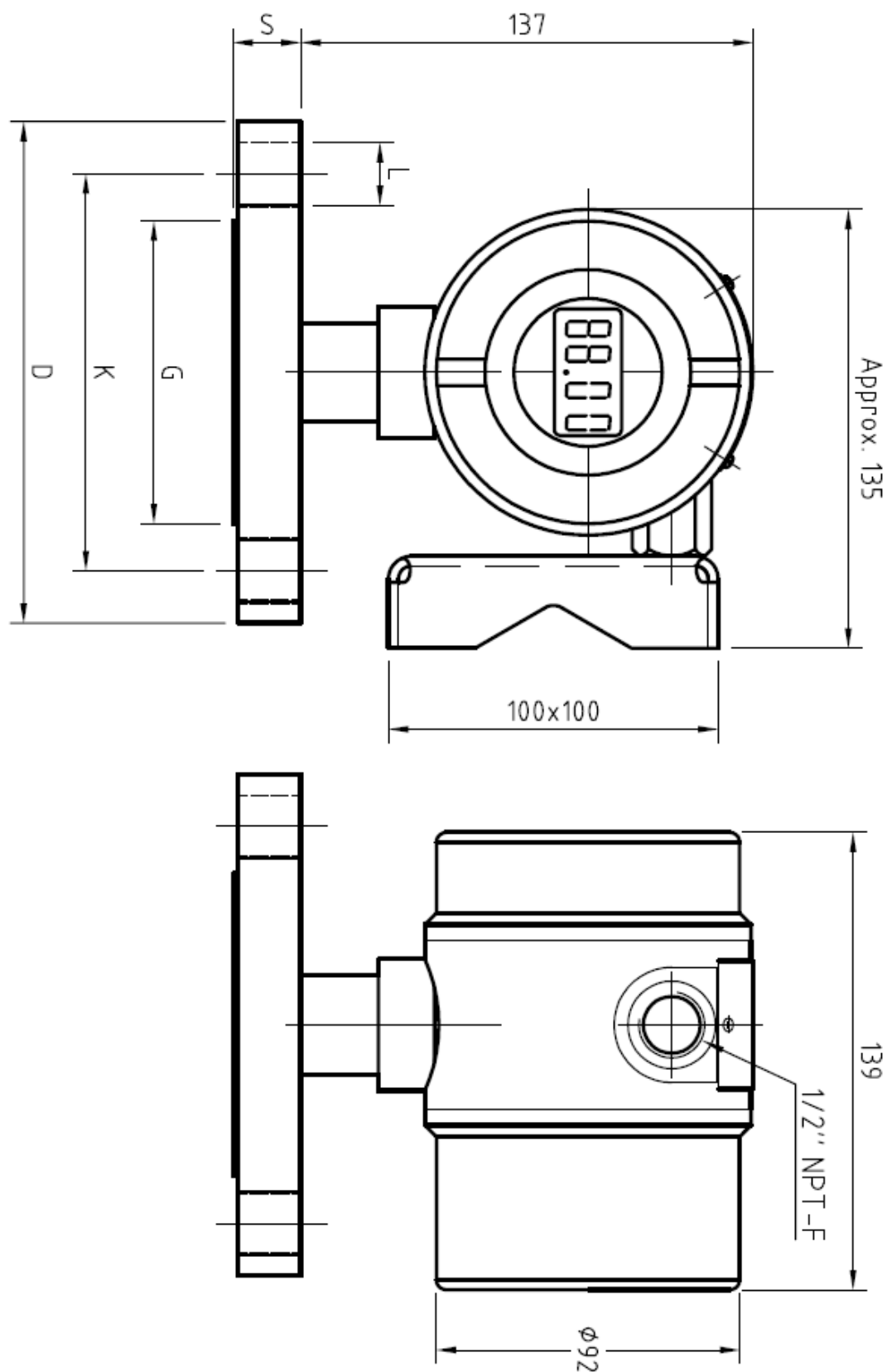
Figura 5 – Flanged connections UNI, ASME etc.
