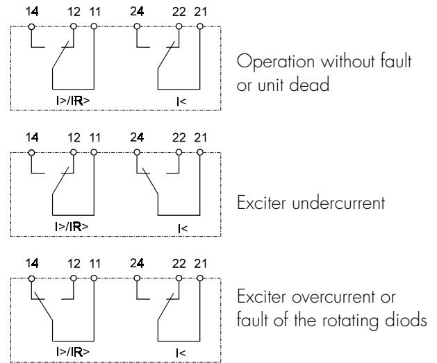
Fig. 2.2: Contact positions of the output relays
