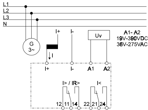
Fig. 2.1: Connections
