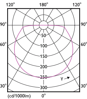
Light Distribution Diagram - LS161 COB LED12 13W 930 5M 24V
