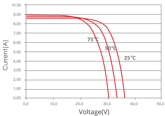
I-V Curves of PV Module 250 Wp at Different Cell Temp. (AM1.5, 1000W/m 2 )
