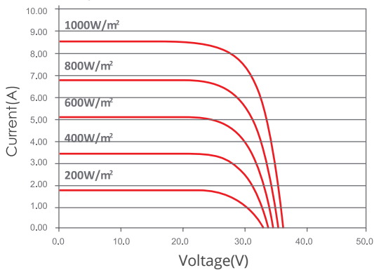
I-V Curves of PV Module 250 Wp (Cell Temp. 25 °C)
