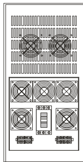
REAR PANEL FRc 1002C3 & FRc 1502C3
