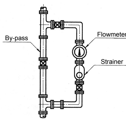
Vertical Installation (Flow Direction : Bottom ⇒ Top)
