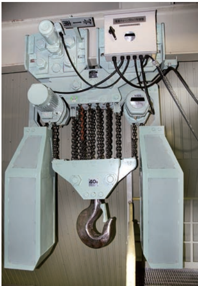
EMT-MH-5 40ton (Special version)
