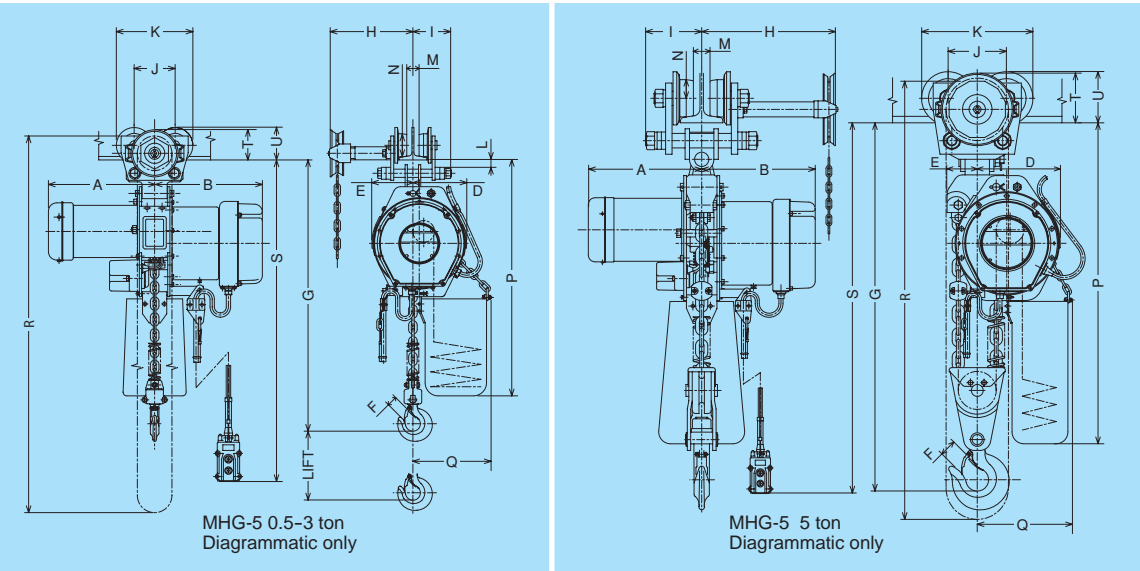
STANDARD SPECIFICATIONS : MHG-5 Electric Chain Hoist with Geared Trolley & MHP-5 Electric Chain Hoist with Plain Trolley
