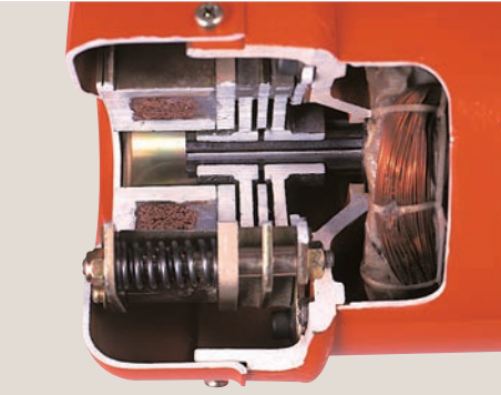
Extra powerful electro-magnetic brake
