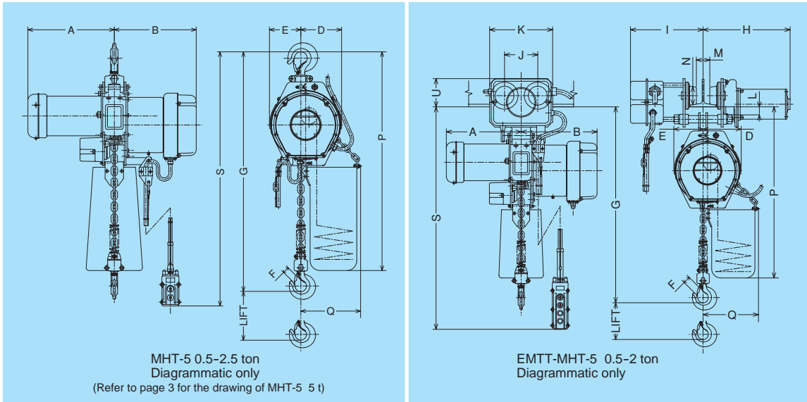
STANDARD SPECIFICATIONS : MHT-5 Two-Speed Electric Chain Hoist (Single-voltage)
