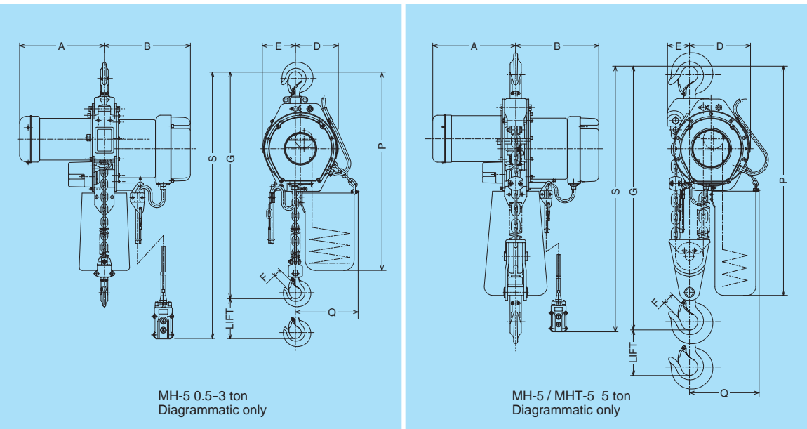
STANDARD SPECIFICATIONS : MH-5 Electric Chain Hoist
