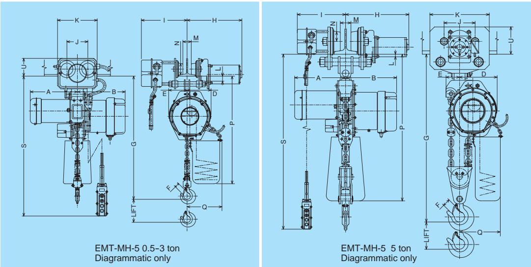
STANDARD SPECIFICATIONS : EMT-MH-5 Electric Chain Hoist with Electric Trolley
