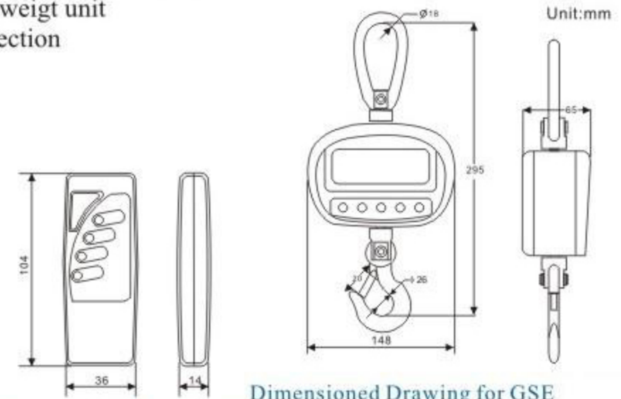
Dimensioned Drawing for Remote Control
