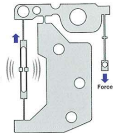
Double-Ended tuning fork (DETF) vibrator
