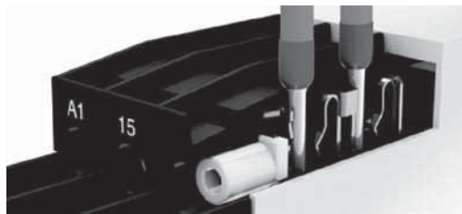
"Easy Connect Technology " Type CM-XXX.xxP
