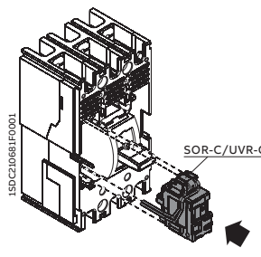
Three-pole circuit-breaker
