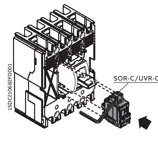
Four-pole circuit-breaker
