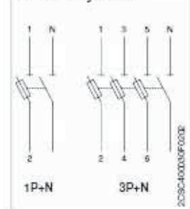
Electrical symbols
