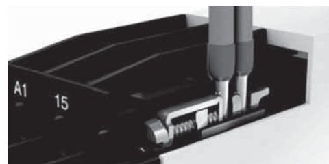
"Double Chamber Cage Connection Terminal" Type CM-XXX.xxS
