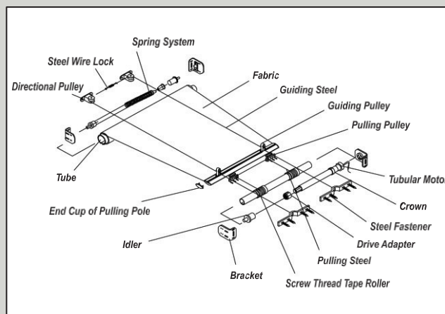
* SKYLIGHT SPRING SYSTEM / FLAT
